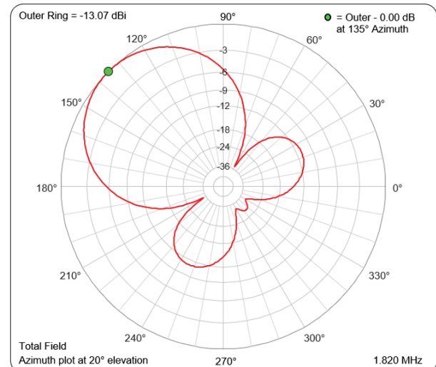
21x21m footprint for 160m/80m with RDF 12.29dB
